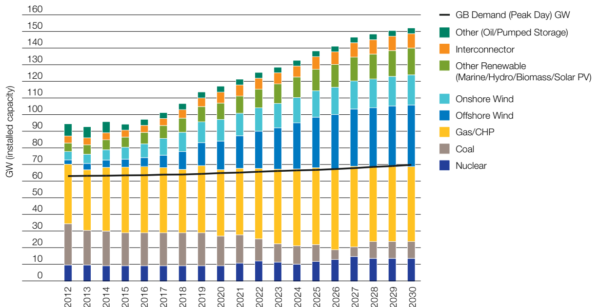
Figure 27. Demand and Generation Background: Gone Green
