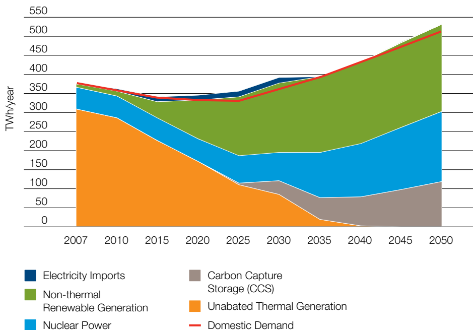
Figure 60. UK Electricity demand and generation
