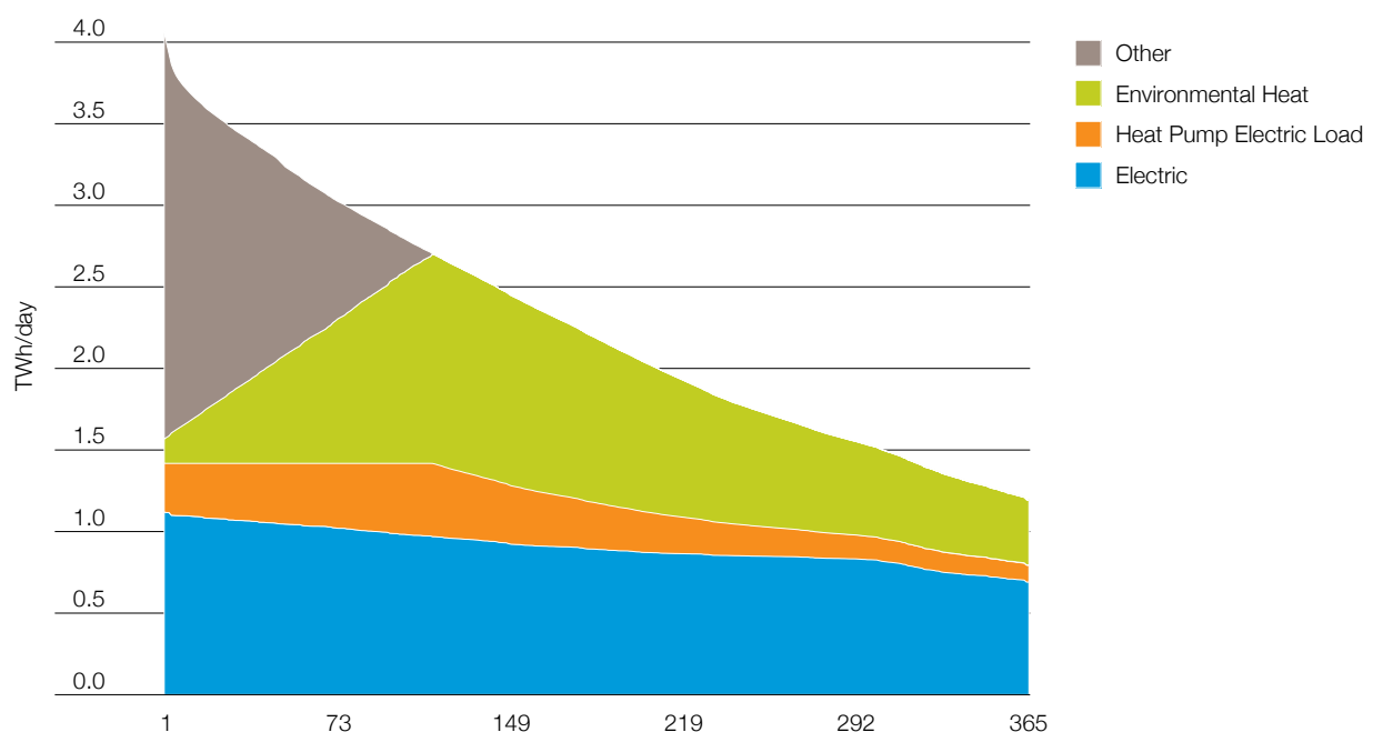
Figure 9. Electricity and heat load duration curves
