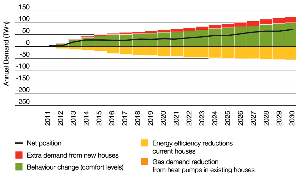
Figure 31. Changes in domestic gas demand: Slow Progression
