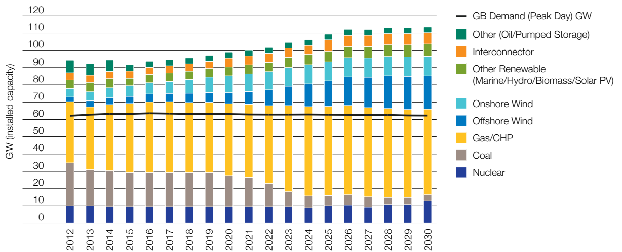
Figure 26. Demand and Generation Background: Slow Progression
