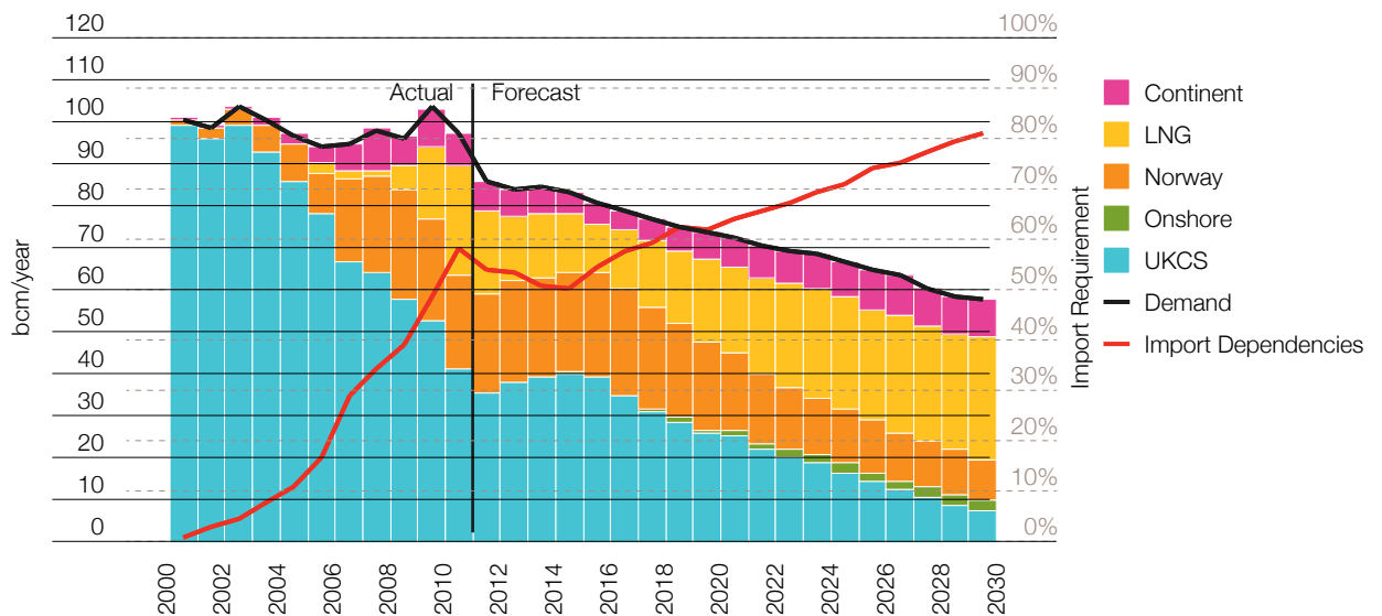
Figure 45. Annual Gas Supply: Gone Green
