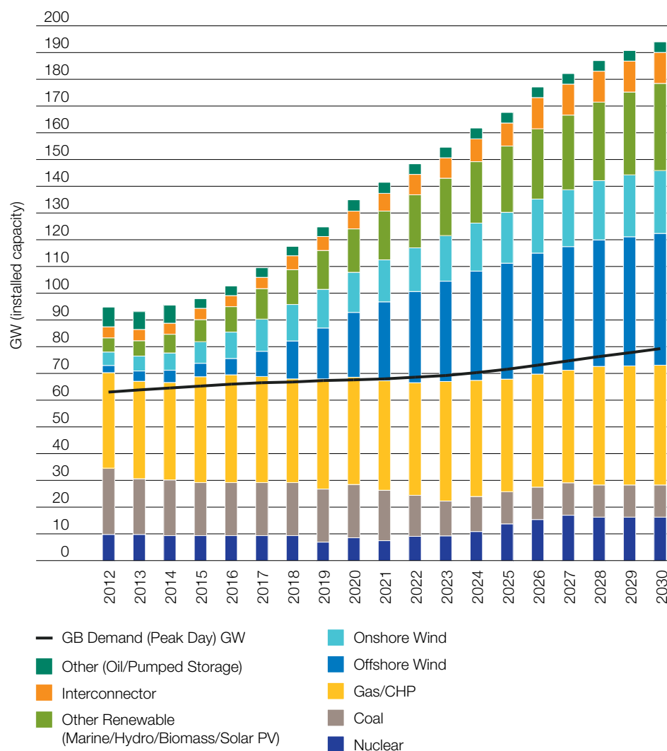
Figure 28. Demand and Generation Background: Accelerated Growth
