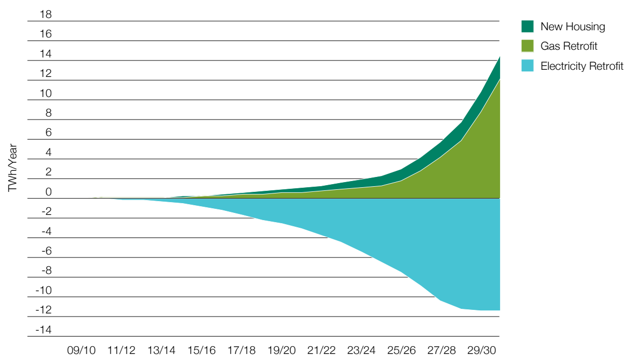
Figure 7. Changes in electricity demand due to domestic heat pumps: Gone Green
